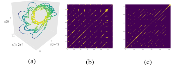
Figure 1: (a) Reconstructed PS ( m = 3 , \tau = 7 ) and (b) RP ( \epsilon = 0.15 , Manhattan norm) of 30ms frame corresponding to vowel /e/. (c) RP of Lorenz96 system displaying chaotic behavior [29]
